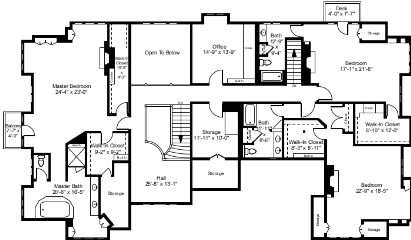
Second Floor Plan Ceiling Height = 8'-0"
